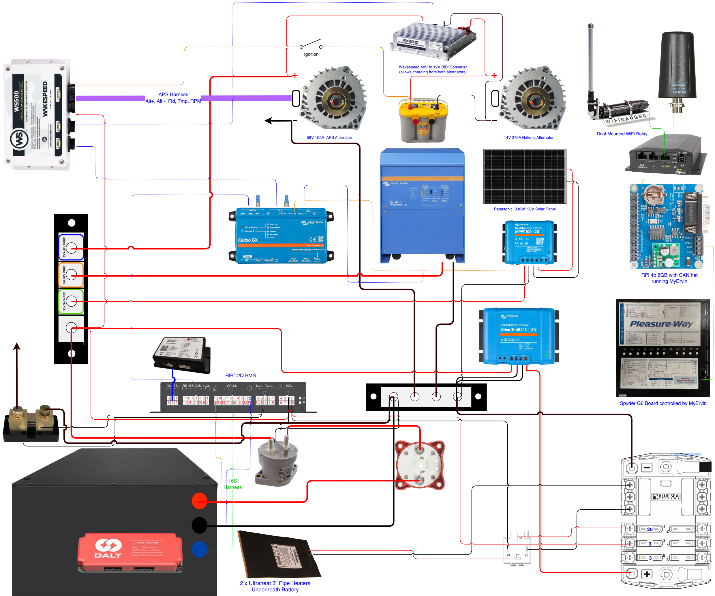
16S1P 51.2V 15.3kWh LiFePO4 with Daly 16S Active Balancer
